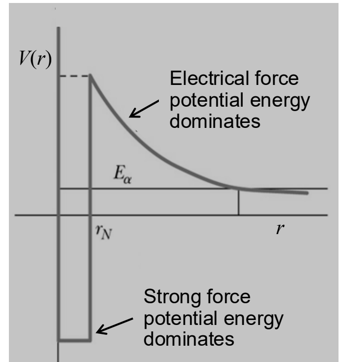
\alpha -particle potential energy curve
