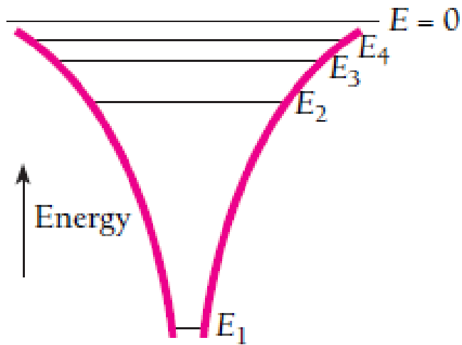
Coulombic Potential
