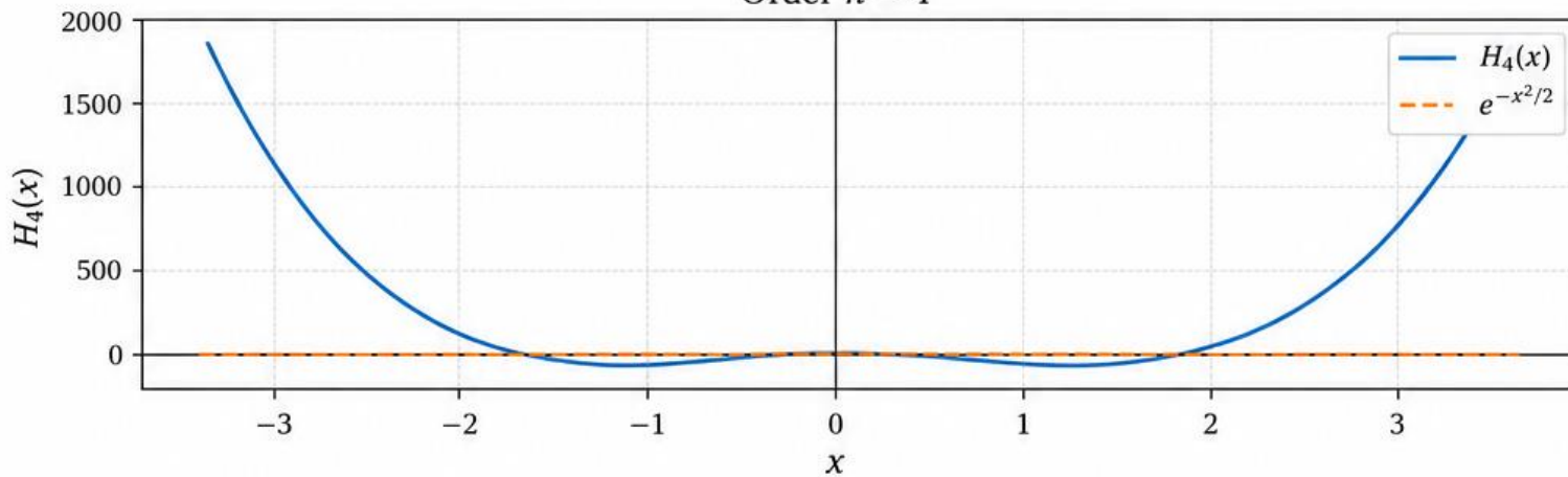
Order n = 4
