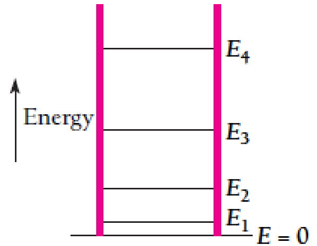
Square well Potential
